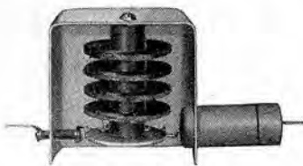
CUT AWAY VIEW OF FOUR PI. R. F. PLATE CHOKE.
