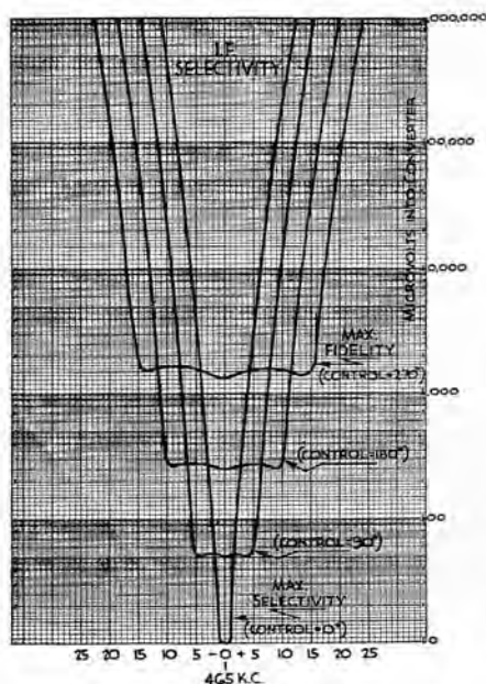
Selectivity Curve
